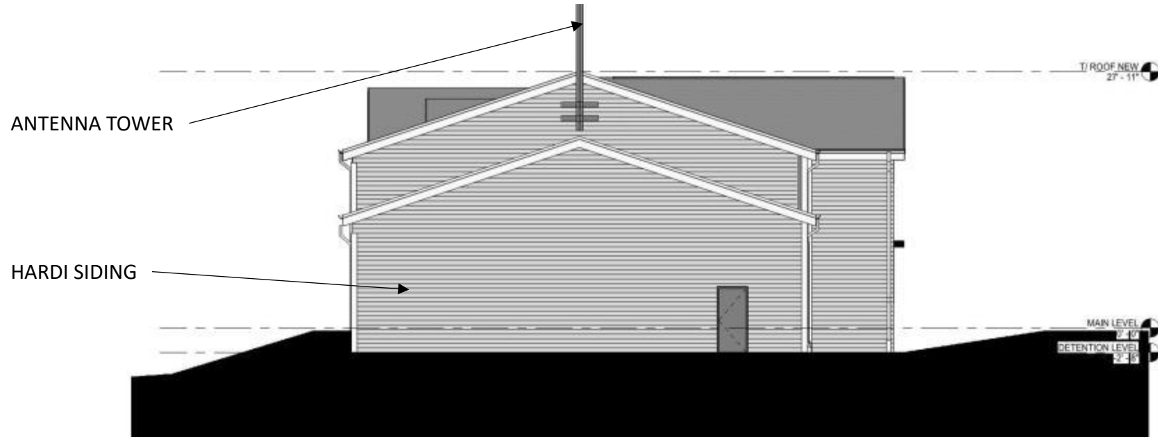
EAST ELEVATION
